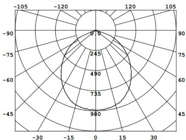
Intensity(unit:cd) C0-180
